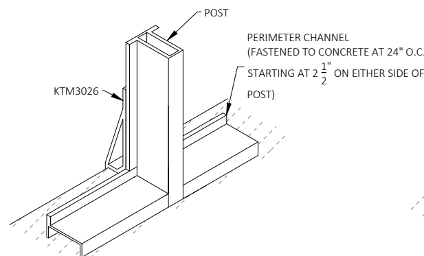
BEFORE INSTALLATION OF PERIMETER CHANNEL
