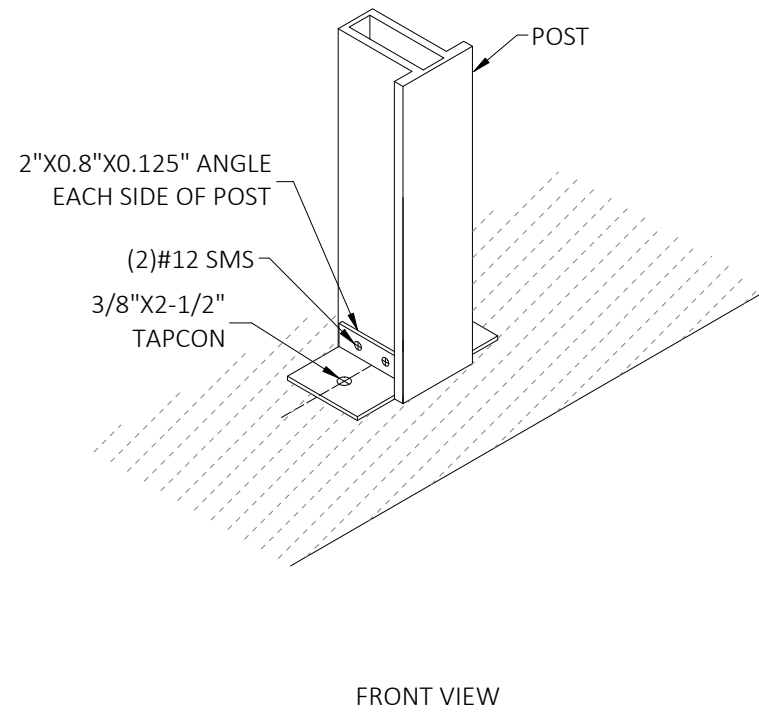
BEFORE INSTALLATION OF PERIMETER CHANNEL
