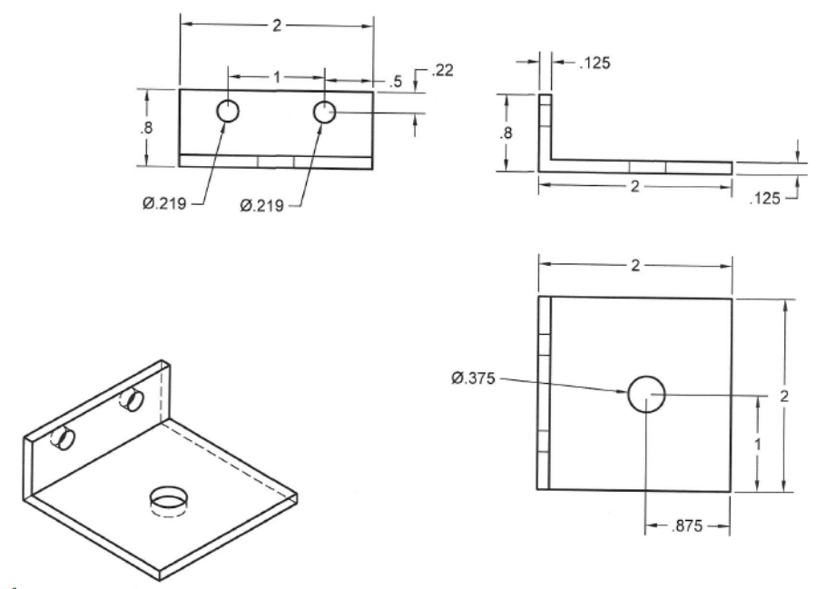
2"X0.8"X0.125" ANGLE
