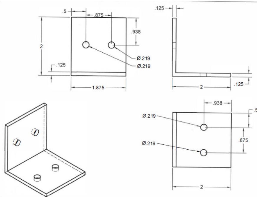
2"X2"X0.125" ANGLE
