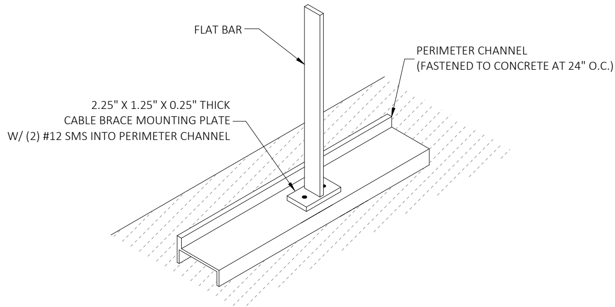
FLAT BAR FASTENING DETAILS SCALE : N.T.S
