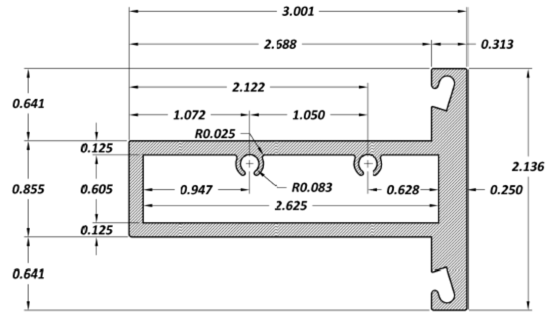
SECTION B
